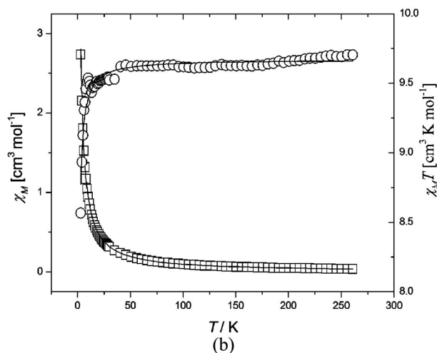
Figure 13. Temperature dependence of \chi_M T and \chi_M for 2 (a) and 3 (b). The solid line represents the theoretical values based on Equation (1) described in the text.
